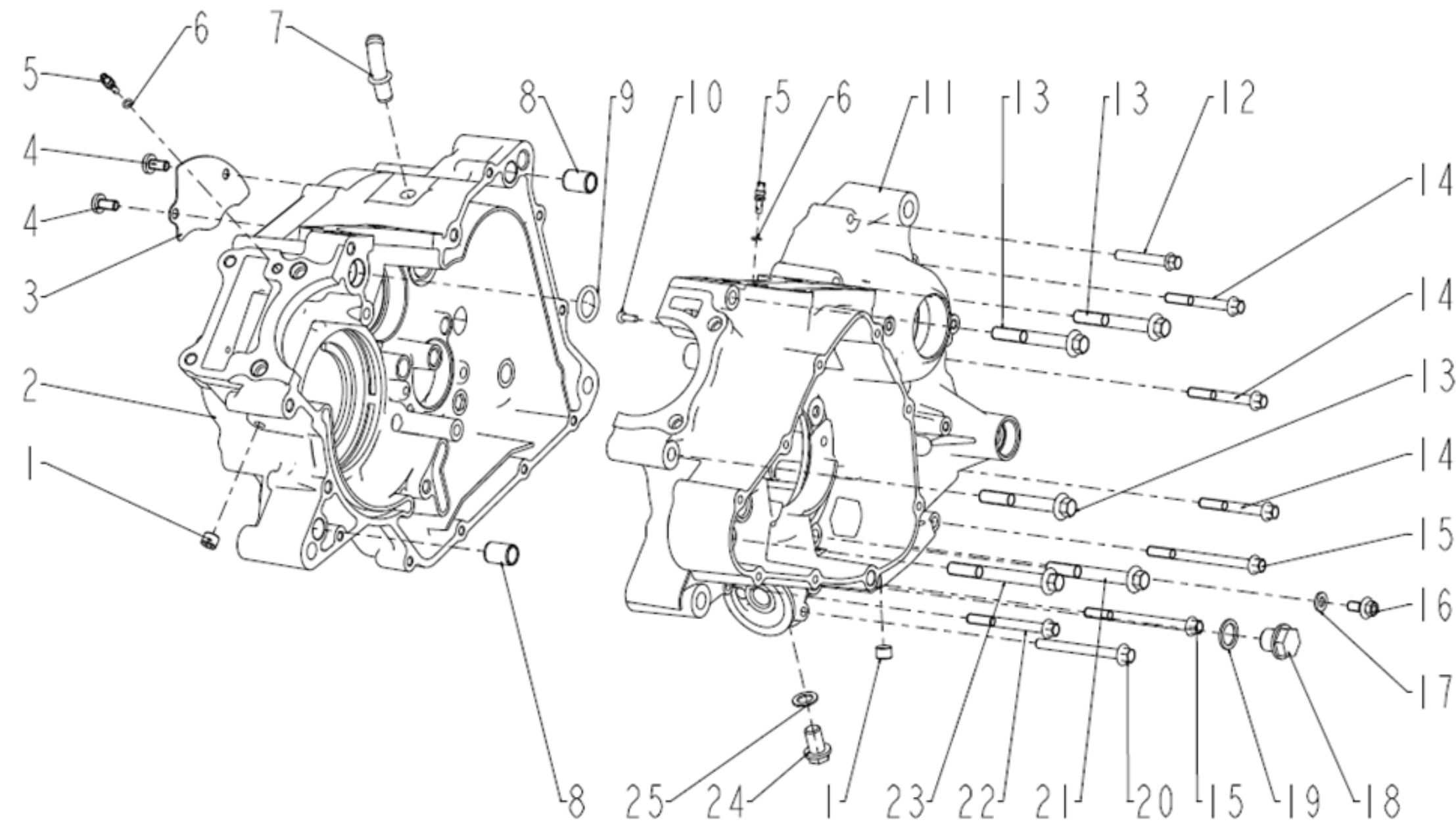
E07 CRANKCASE ASSY(曲轴箱分总成)
