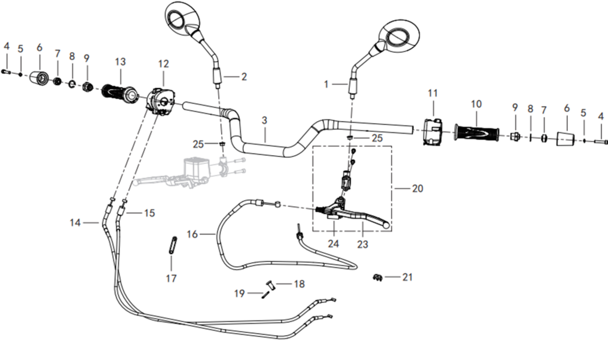
F01 操纵总成 CONTROL ASSY.
