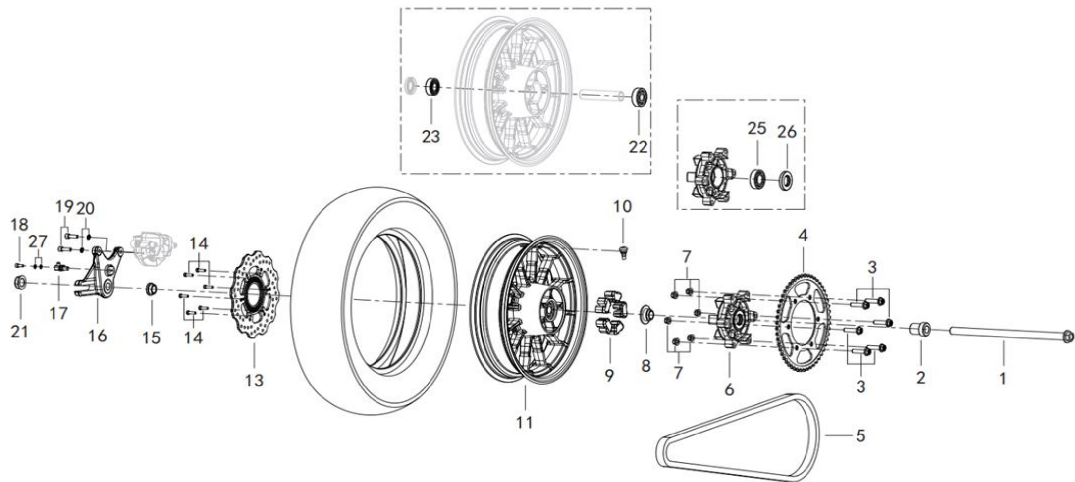
F09 后轮总成 REAR WHEEL ASSY.
